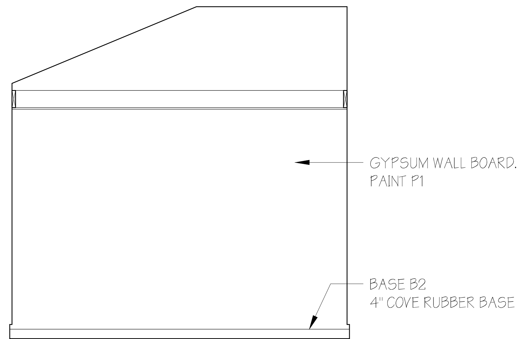
SOUTH ELEVATION
