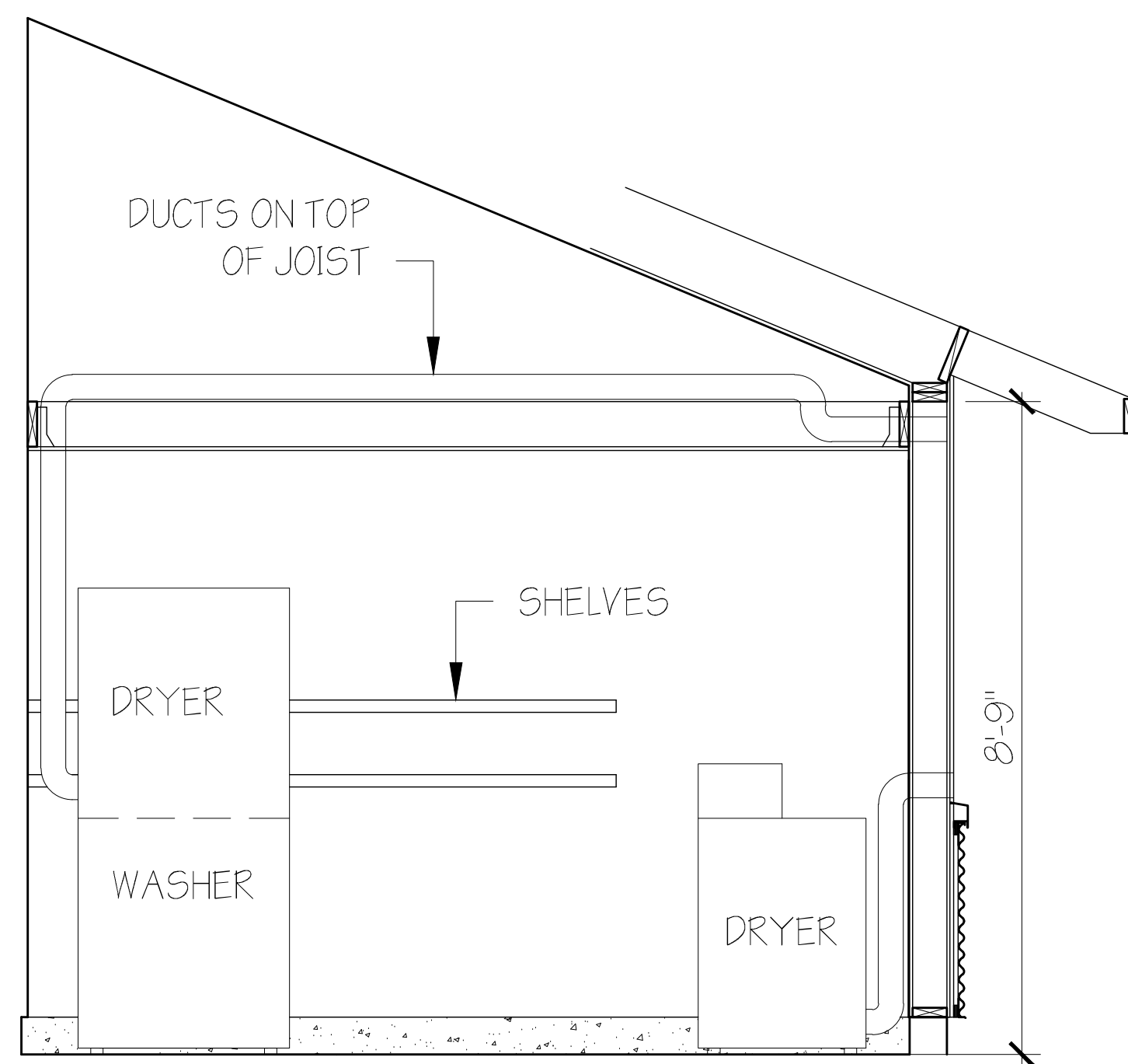
NORTH ELEVATION
