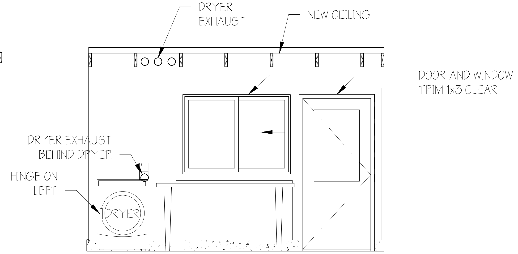
EAST ELEVATION
