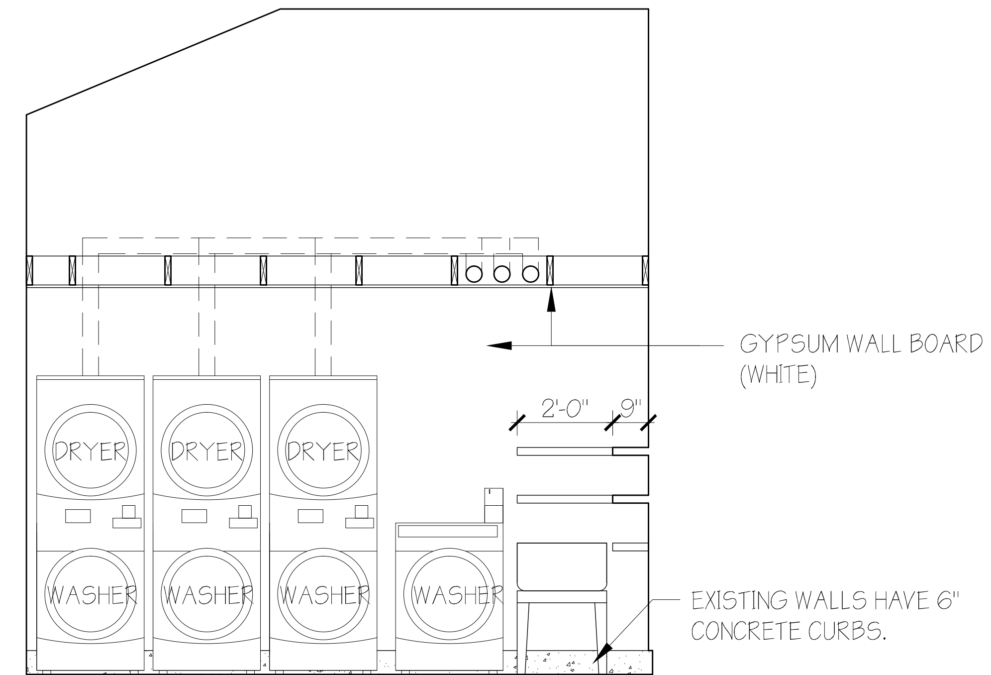
WEST ELEVATION
